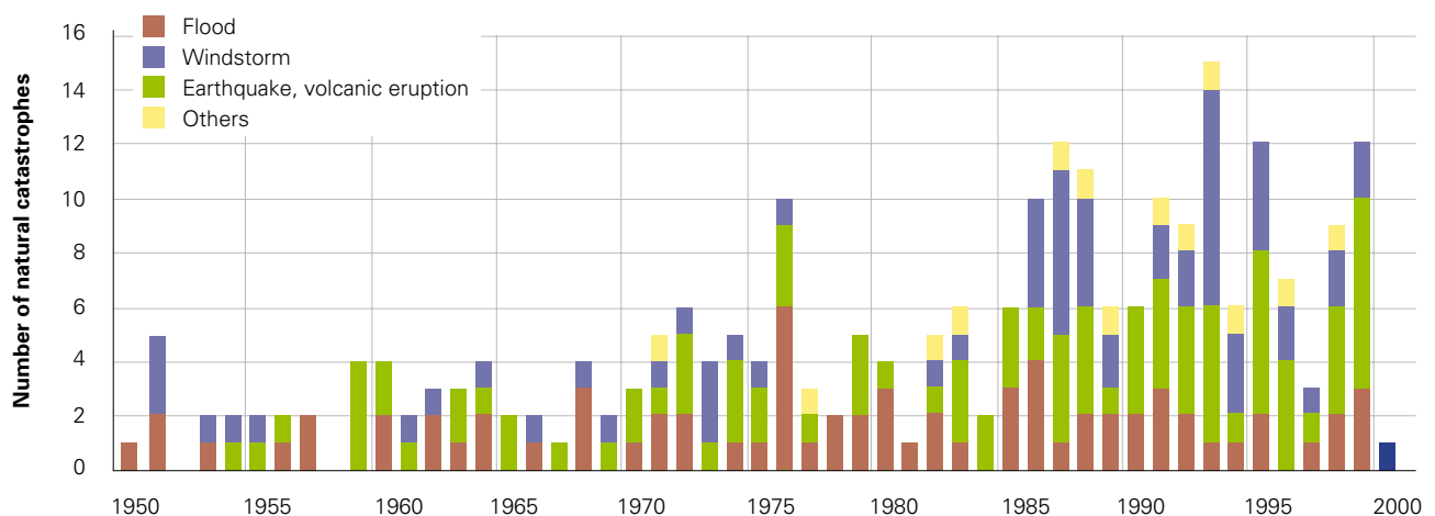
Figure 11.2: Trends in major natural catastrophes, 1950–2000
