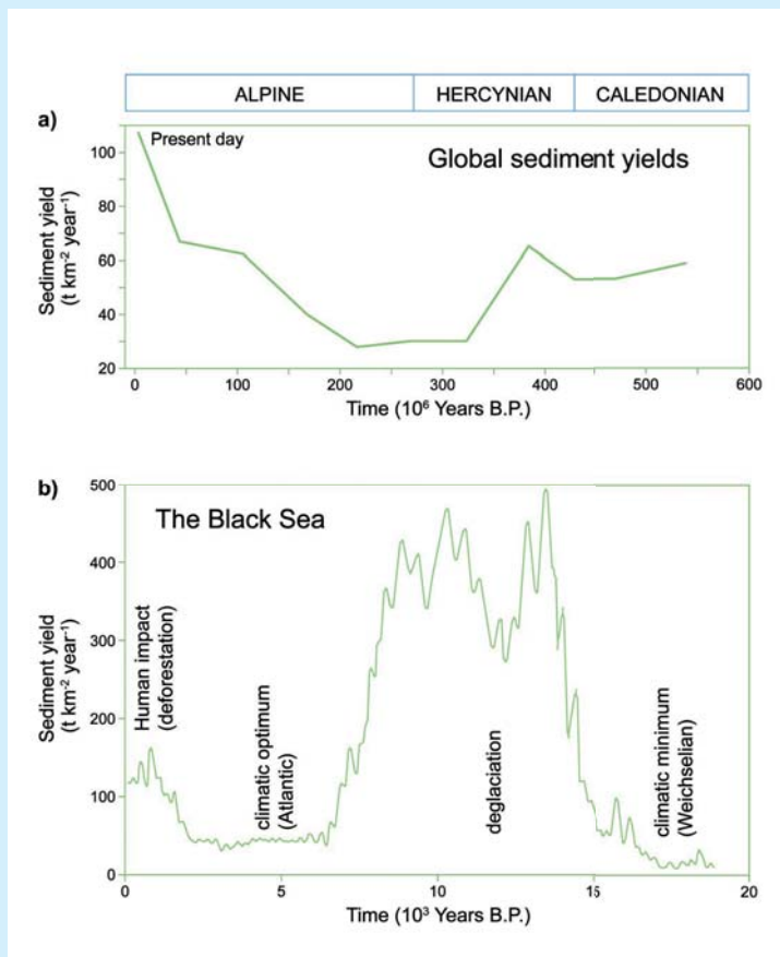
Figure 1 Orogenic cycles
