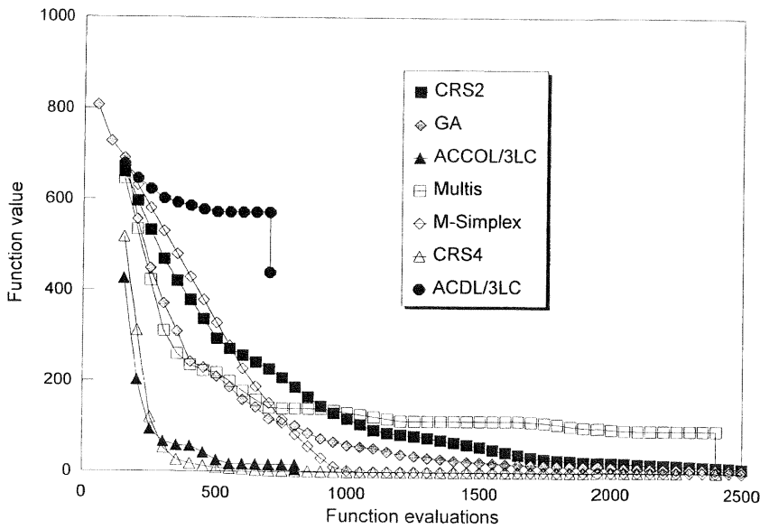
Figure 5f. Griewank function (10-var.)
