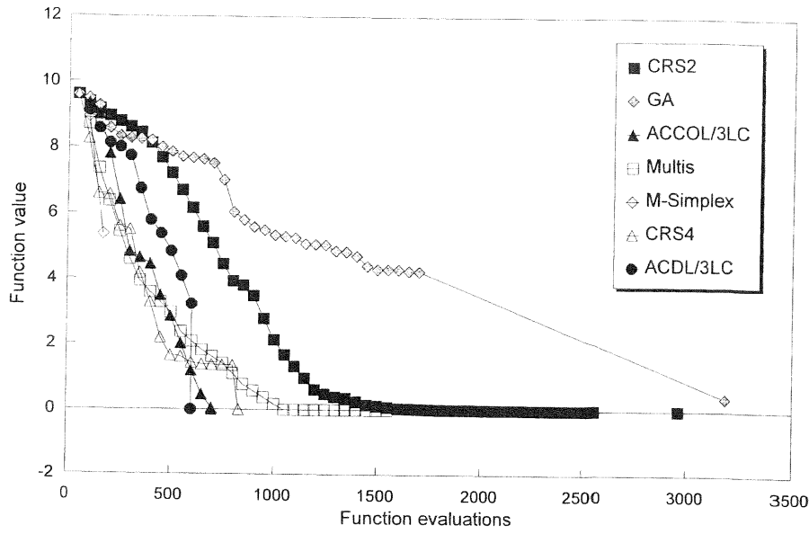
Figure 3e. Shekel10 function (4-var.)
