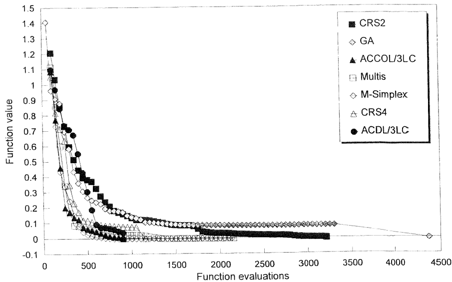
Figure 3d. Hartman6 function (6 var.)
