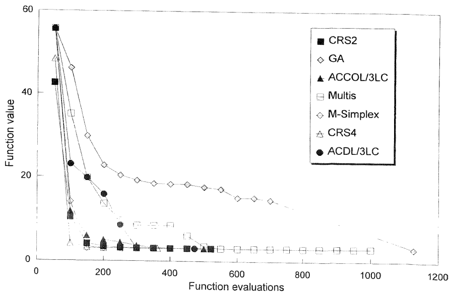
Figure 3b. Goldstein-Price function (2-var.)
