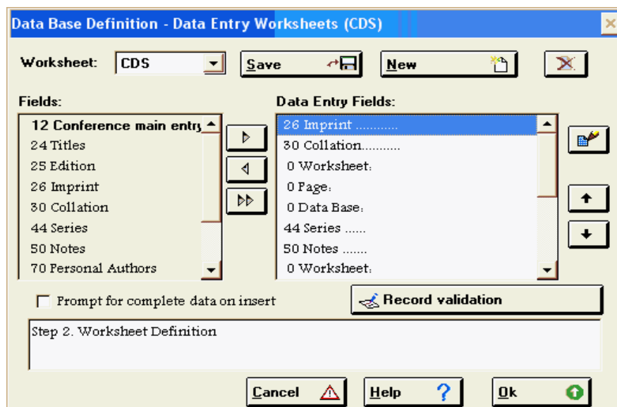
Figure 14 - FMT Editor
