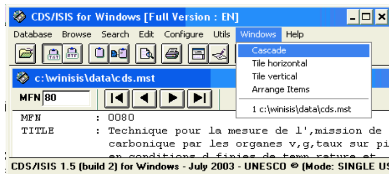
Figure 23 - Windows Menu
