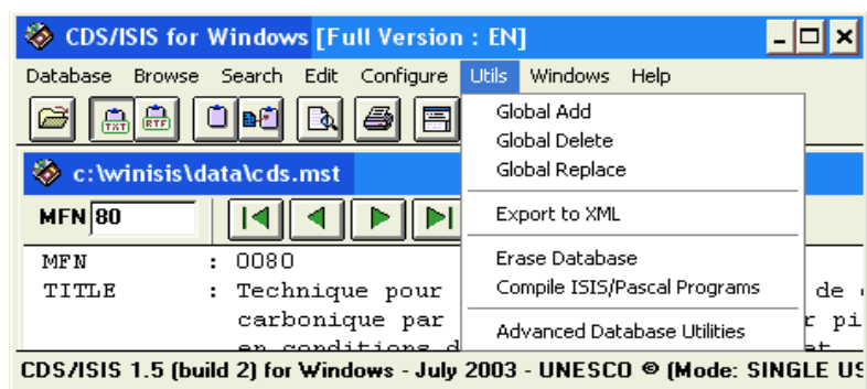
Figure 21 - Utilities Menu
