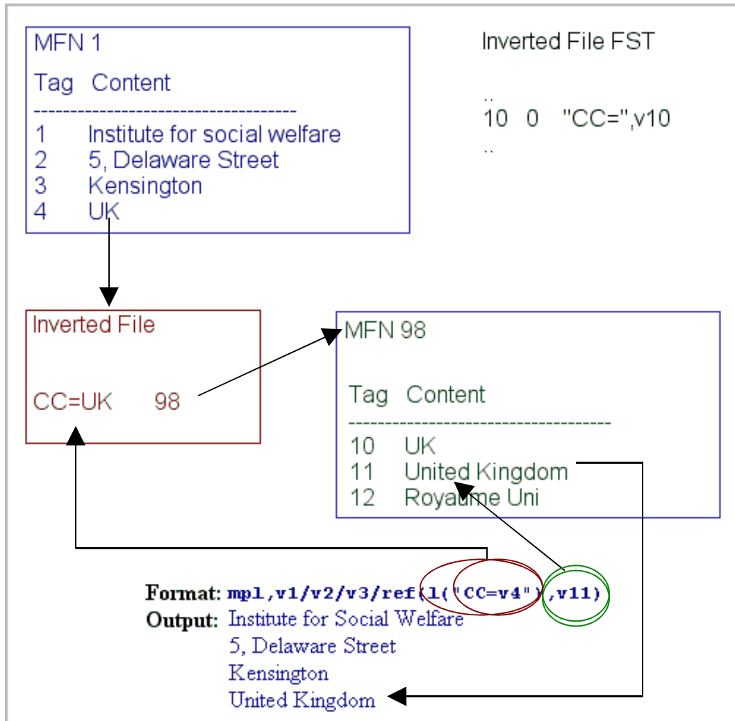
Figure 56 - REF example
