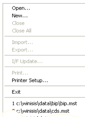
Figure 9 - Database Menu
