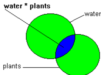
Figure 54 - Logical AND
