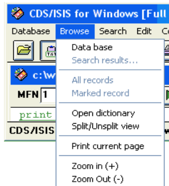
Figure 10 - Browse Menu
