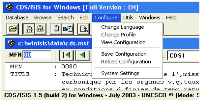
Figure 17 - Configure Menu
