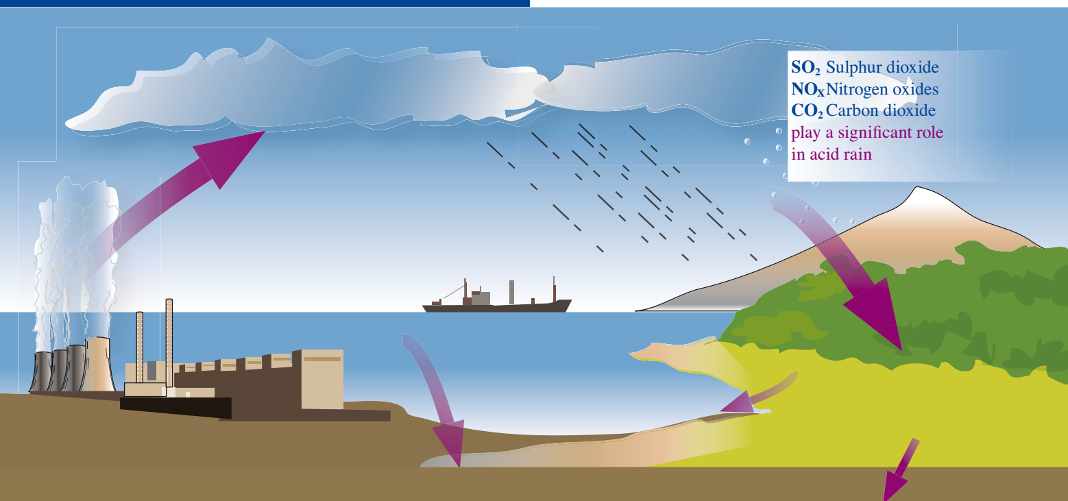
Figure 11 Acid rain
