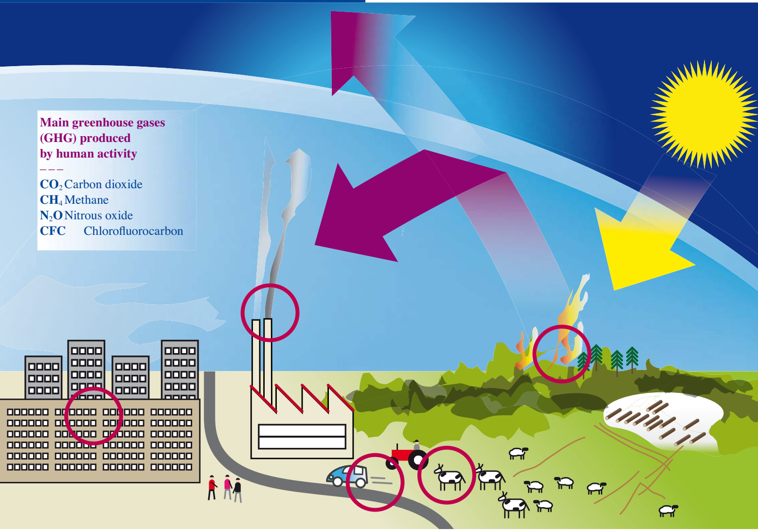
Figure 10 The greenhouse effect
