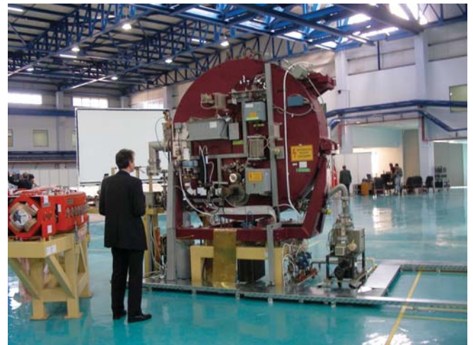
The microtron in the SESAME experimental hall. The first electron beam was produced on 14 July 2009.
