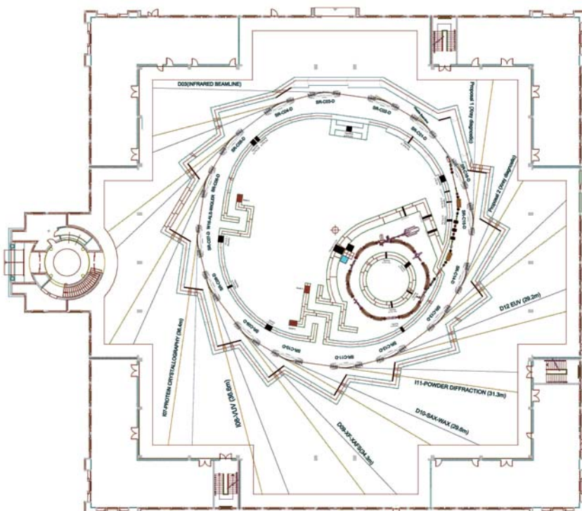
The microtron in the SESAME experimental hall. The first electron beam was produced on 14 July 2009.
