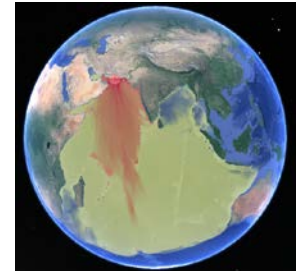
Maximum wave height map for Makran magnitude 9.0 Scenario (BMKG)
