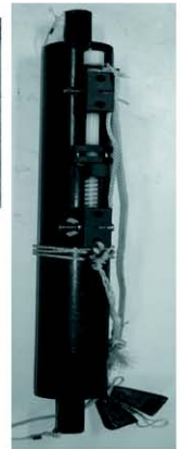
Water sampler
