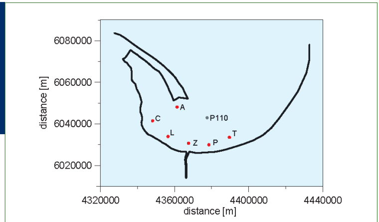
FIGURE 2 Location of modelled sites in the Gulf of Gdańsk in the 1994 reanalysis. Robakiewicz, 2007
