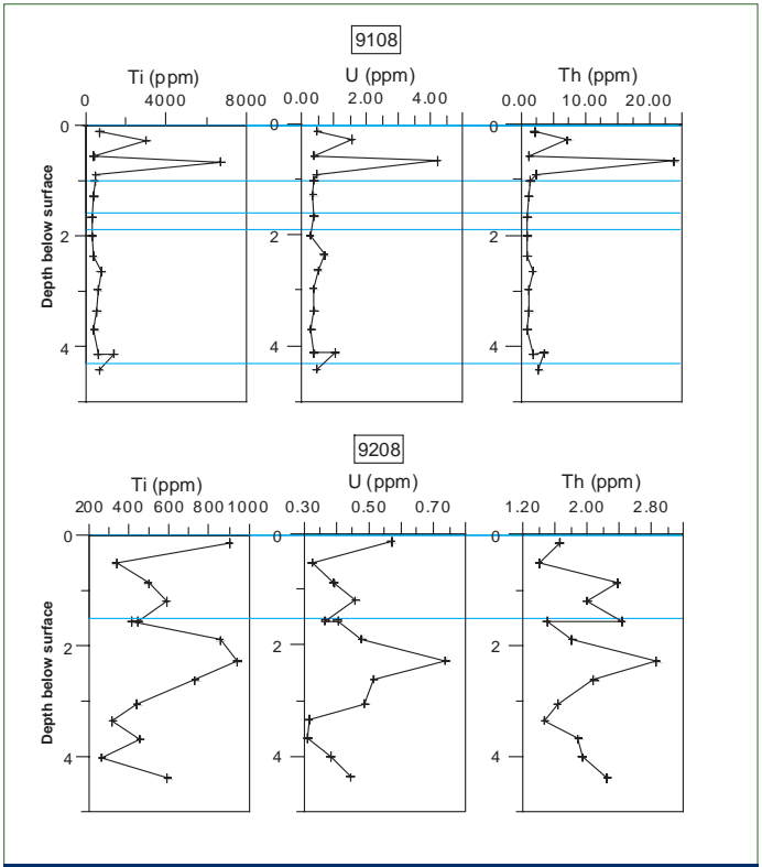
FIGURE 12 Indicator elements for heavy minerals. Accumulations of heavy minerals were found at the top of core 9108, indicating winnowing, whereby quartz and feldspars are transported as heavy minerals lag.
