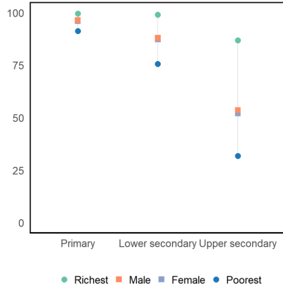
Completion rate, 2015
