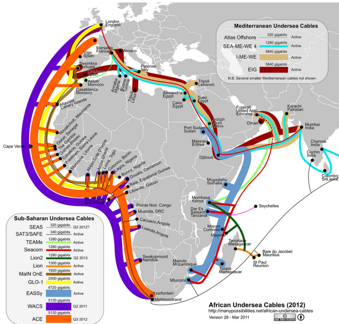
Figure 46. Figure: African Undersea Cables
