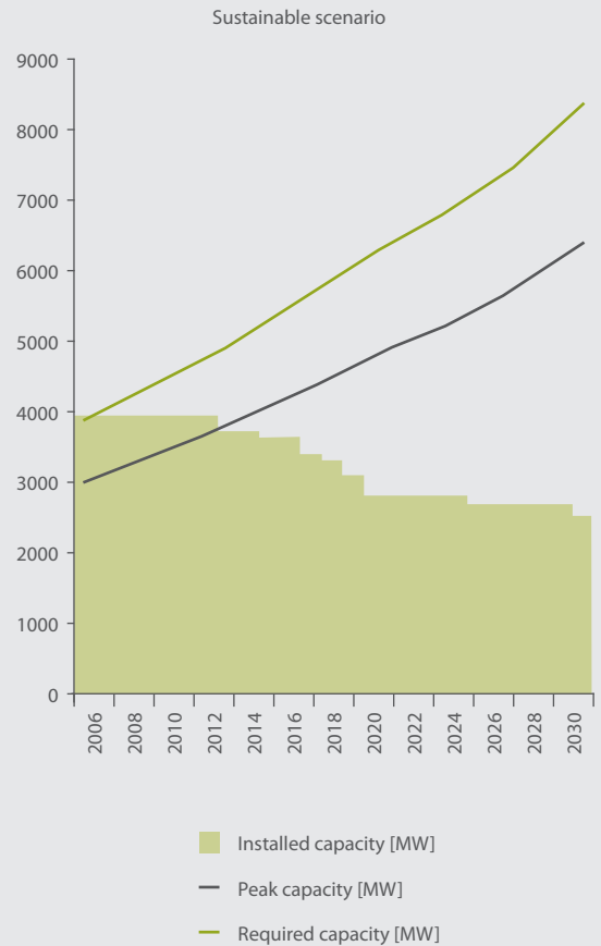
Figure 14-1: Graph indicating the decrease in power generation capacity due to the decommissioning of existing facilities and the required capacity necessary to satisfy demand.
