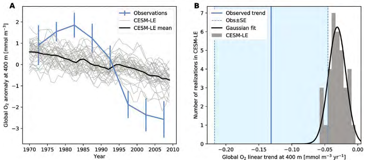
Figure 4.20 Global O 2 trends from observations and CESM-LE. (A) Globally average O 2 concentration at the depth of 400m from 1970 to 2010. The thin solid lines represent individual ensemble members of the CESM-LE, and the thick solid line is the ensemble mean. Blue line is the pentad time series of objectively mapped O 2 dataset based on the World Ocean Database (Ito et al., 2017). Error bars indicate one standard deviation of the pentad data. (B) Histogram of linear O 2 trend at 400 m. The black line is a gaussian fit, and the blue solid line is the observed trend; the dashed lines and shaded region show its uncertainty as measured by one standard error.
