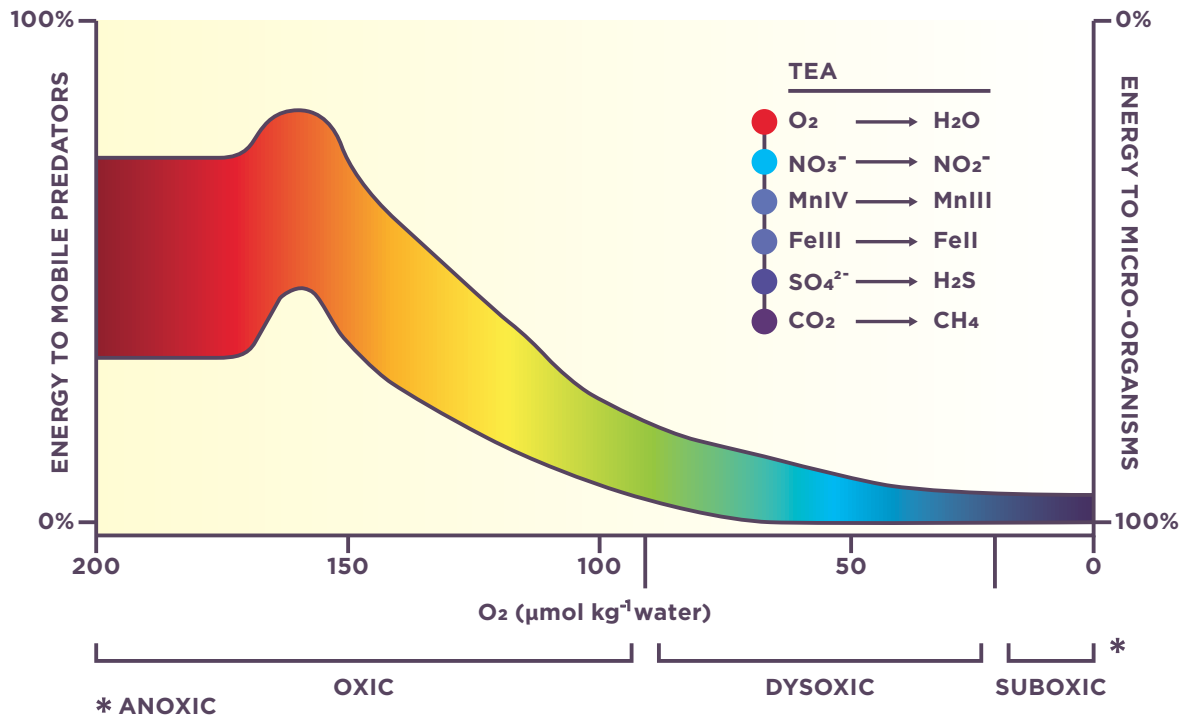
Figure 8.4.2 Oxidic, dysoxic (or hypoxic) and anoxic states of the ocean are defined in relation to oxygen concentration, along with the dominant energetic pathways at each state. From Wright et al. (2012).
