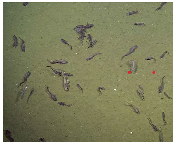
Figure 8.5.3 High density fish aggregations of cusk eel Cherublemma emmelas were observed in the Gulf of California at very low oxygen concentrations ( 1.61 \mu mol kg^{-1} ) (from Gallo et al. 2019). Image from MBARI's ROV Doc Ricketts, red lasers are 29 cm apart.
