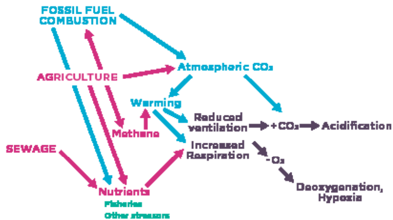
Figure 11.2 Linked causes and mechanisms of oxygen loss. Not shown are pathways for some greenhouse gases such as N 2 O, or feedbacks, including the potential for deoxygenation and warming to increased production of greenhouse gases such as nitrous oxide and methane. Red = major pathways for nutrient sources and effects; blue = major pathways for warming and CO 2 enrichment; green = other stressors that can increase respiration, for example by altering food webs.
