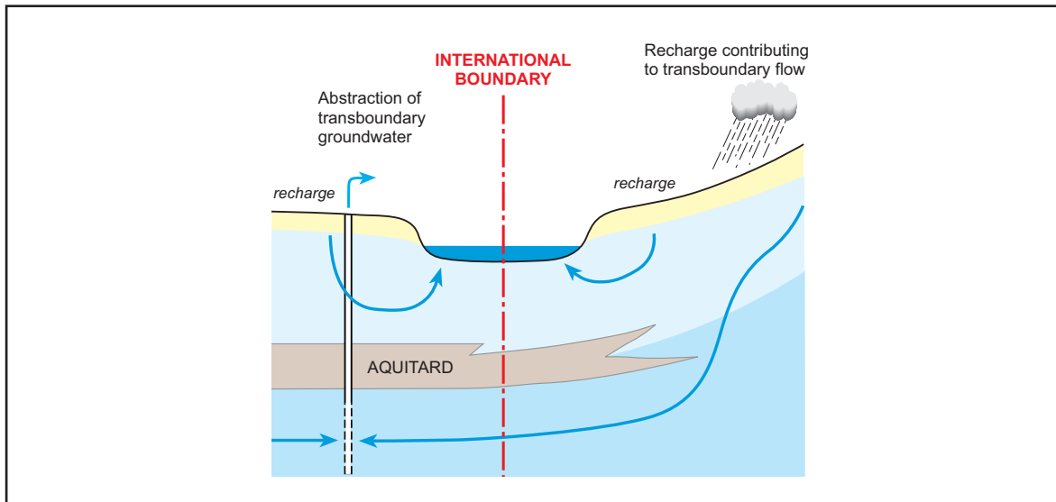
Figure 4. River boundaries over transboundary aquifers
