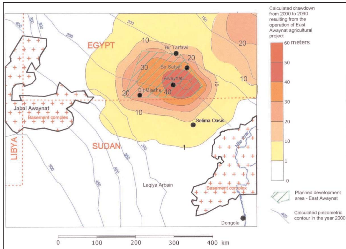
Figure 8. Possible scenario of the spread of the cone of depression (model simulation)
