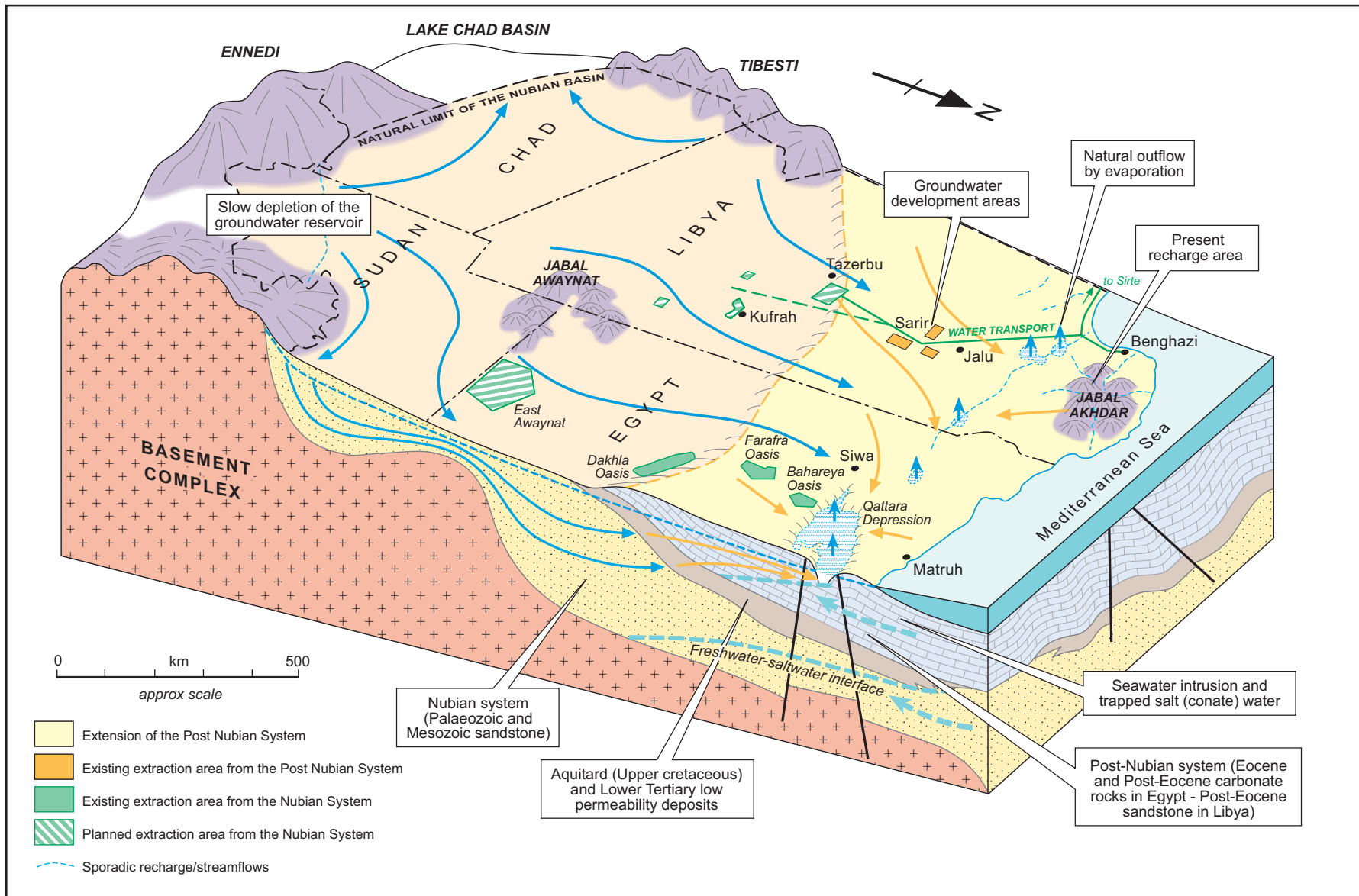
Figure 12. Block diagram of the Nubian Sandstone Aquifer System
